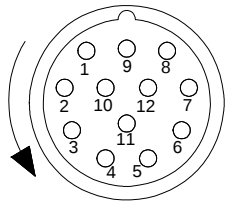
FEMALE END VIEW
